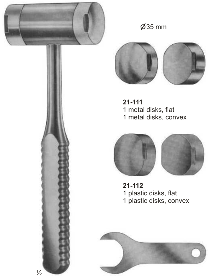
21-113 Wrench
